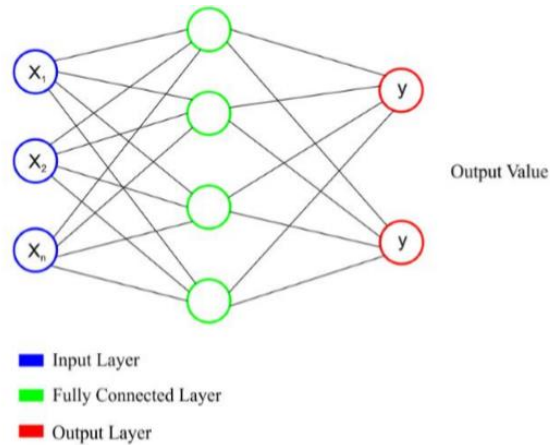
Figure 5 Fully Connected Layer
