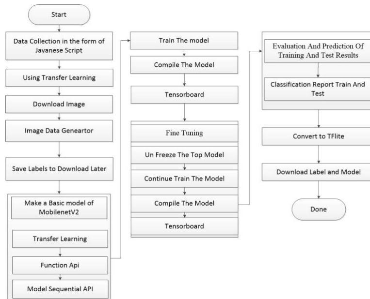
Figure 8 Flowchart of Dataset Training
