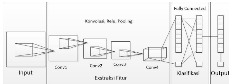
Figure 1 CNN Process Flow
