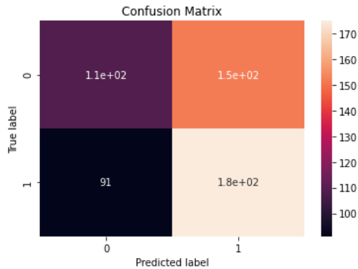
Fig. 1: Confusion Matrix
