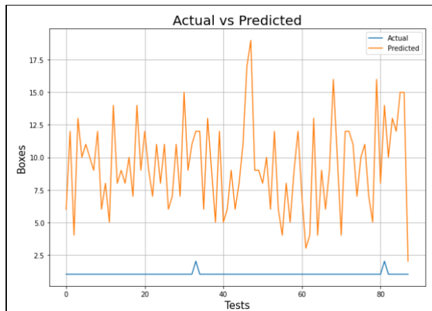
Fig. 3: Actual vs Predicted testing process
